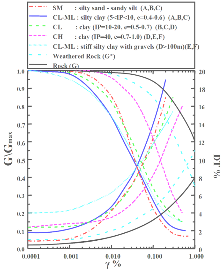
Figure 4: Mean G/G_0 - \gamma - D curves from resonant column and cyclic triaxial tests for all geotechnical formations occur at station TST_018. The curves describe the shear modulus degradation with the shear strain and the respective internal damping increase.
