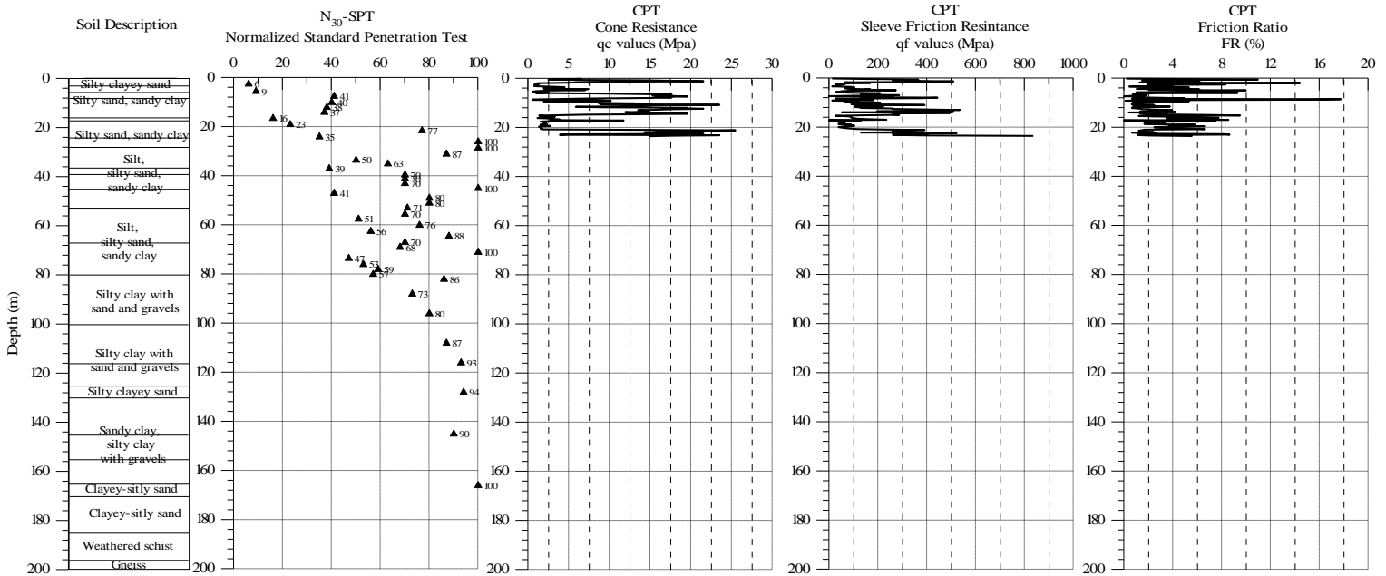
Figure 3: Geotechnical data at station TST_018
