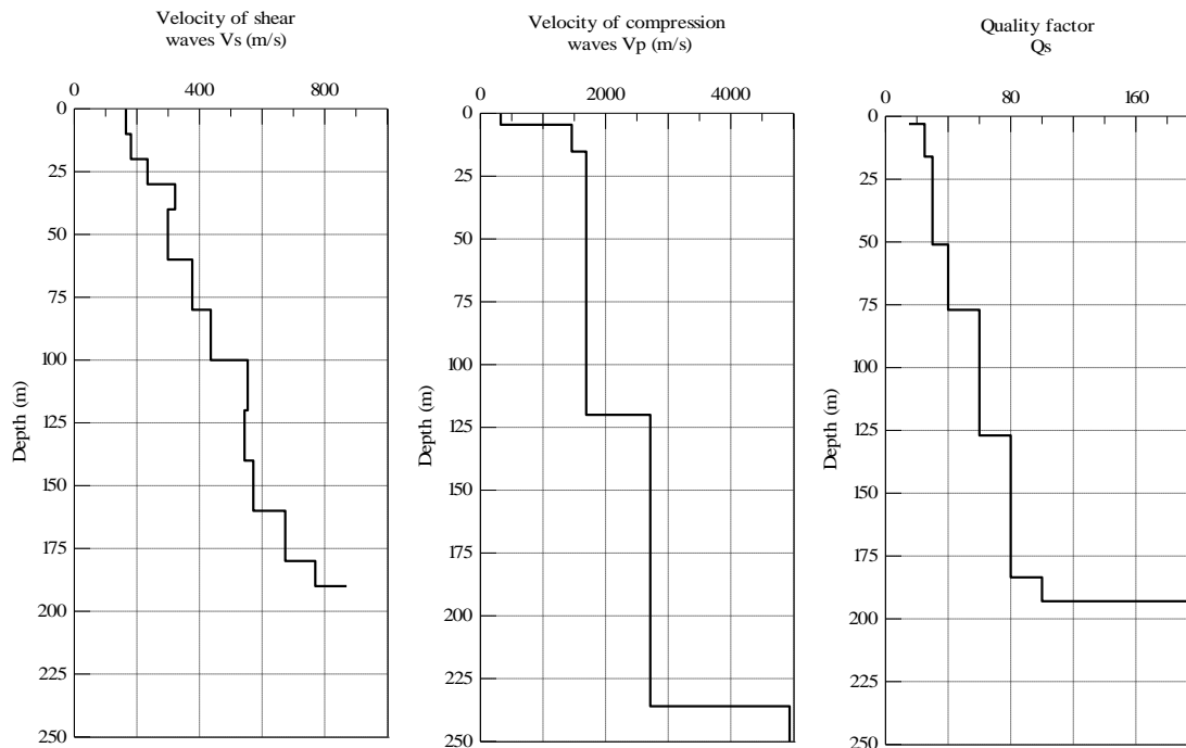
Figure 5: Shear and compression wave velocity and Quality factor values at station TST_018.
